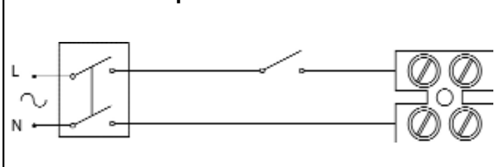
AMF100C with Remote Switch Pull cord to ON position and cut off
